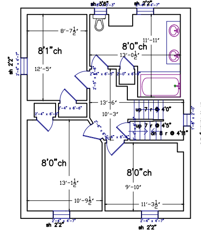
Second Floor - 742sf
