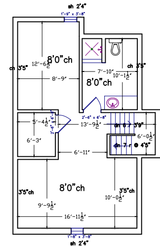
Third Floor - 567sf
