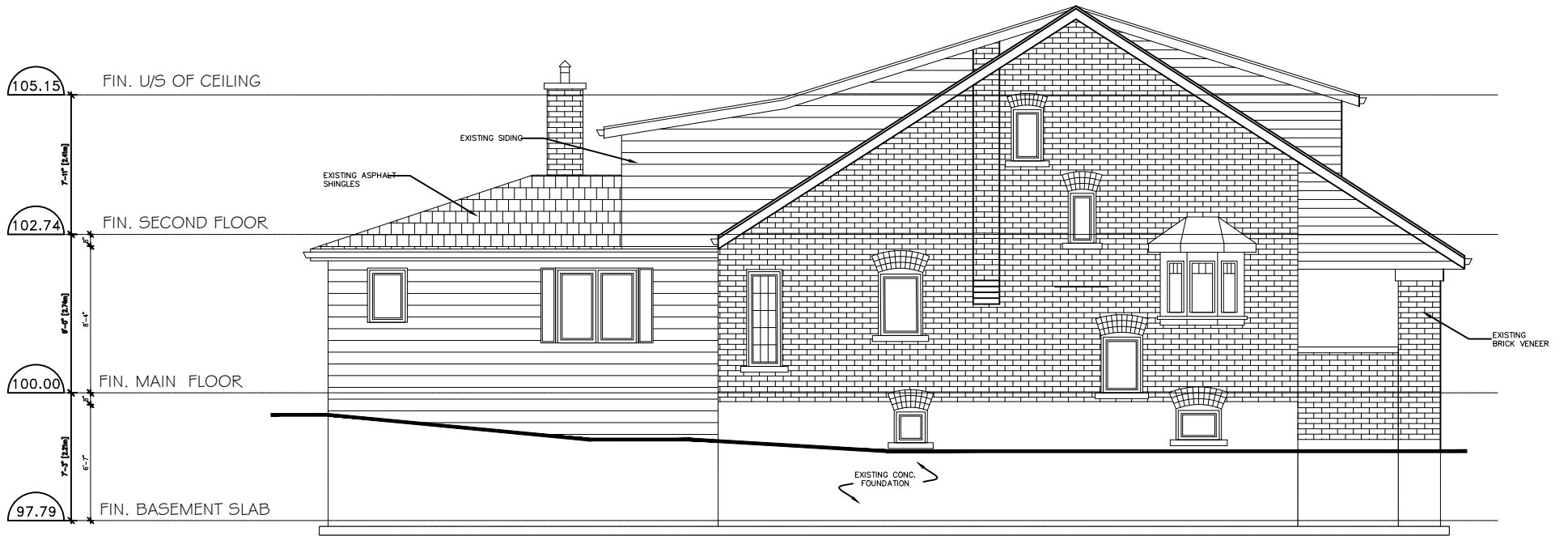
LEFT SIDE (SOUTH) ELEVATION
