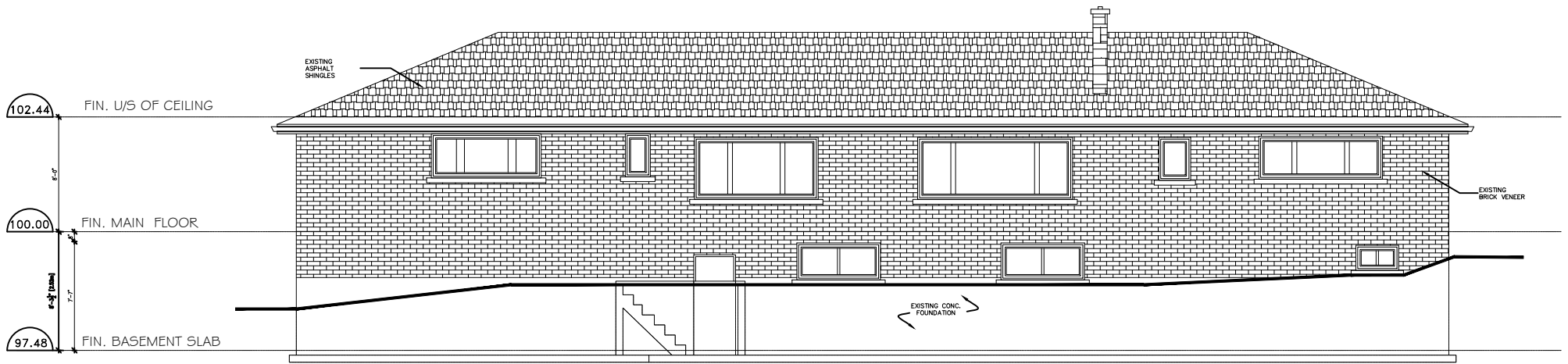
REAR (NORTH) ELEVATION
