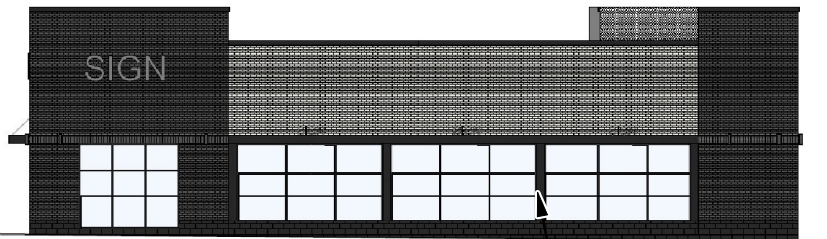
NORTH ELEVATION
