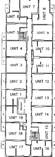
PLAN VIEW SHOWING RESIDENTIAL UNITS 1 TO 19 INCLUSIVE ON LEVELS 5 TO 8 INCLUSIVE
