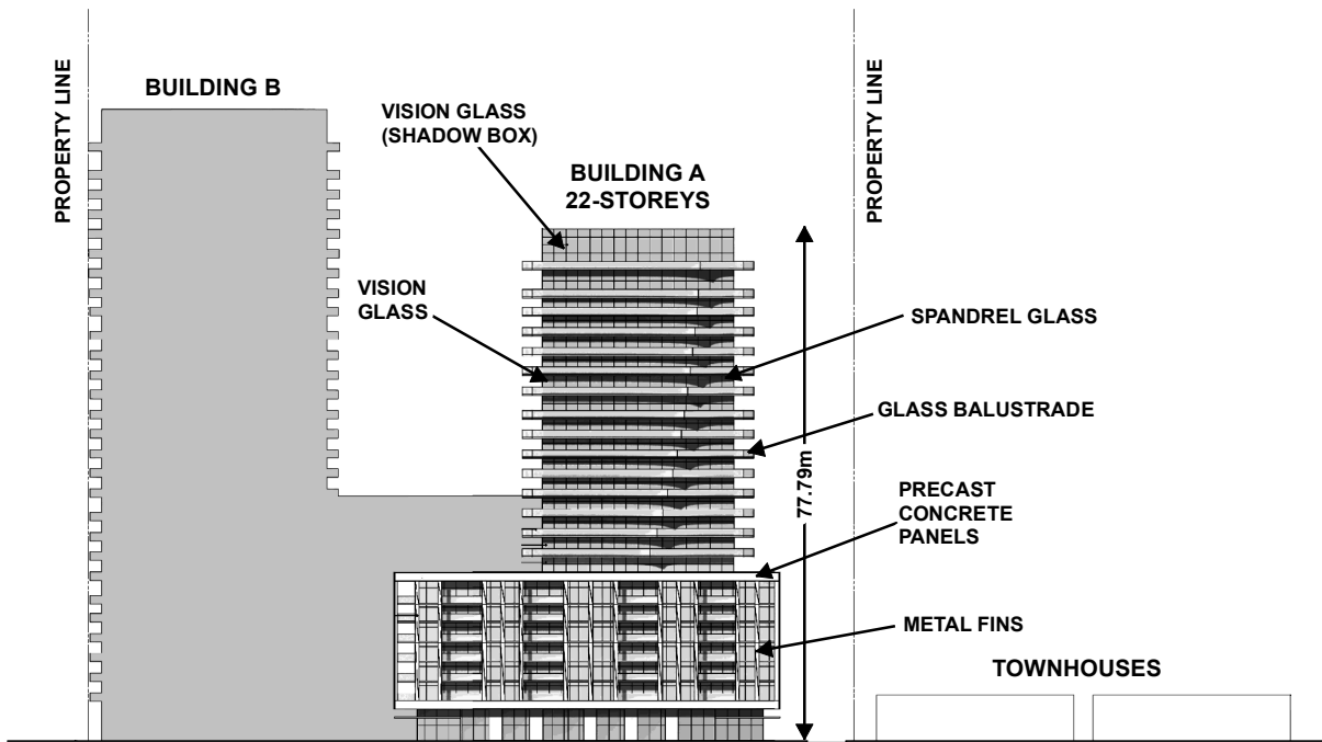
BUILDING A - EAST ELEVATIONS
