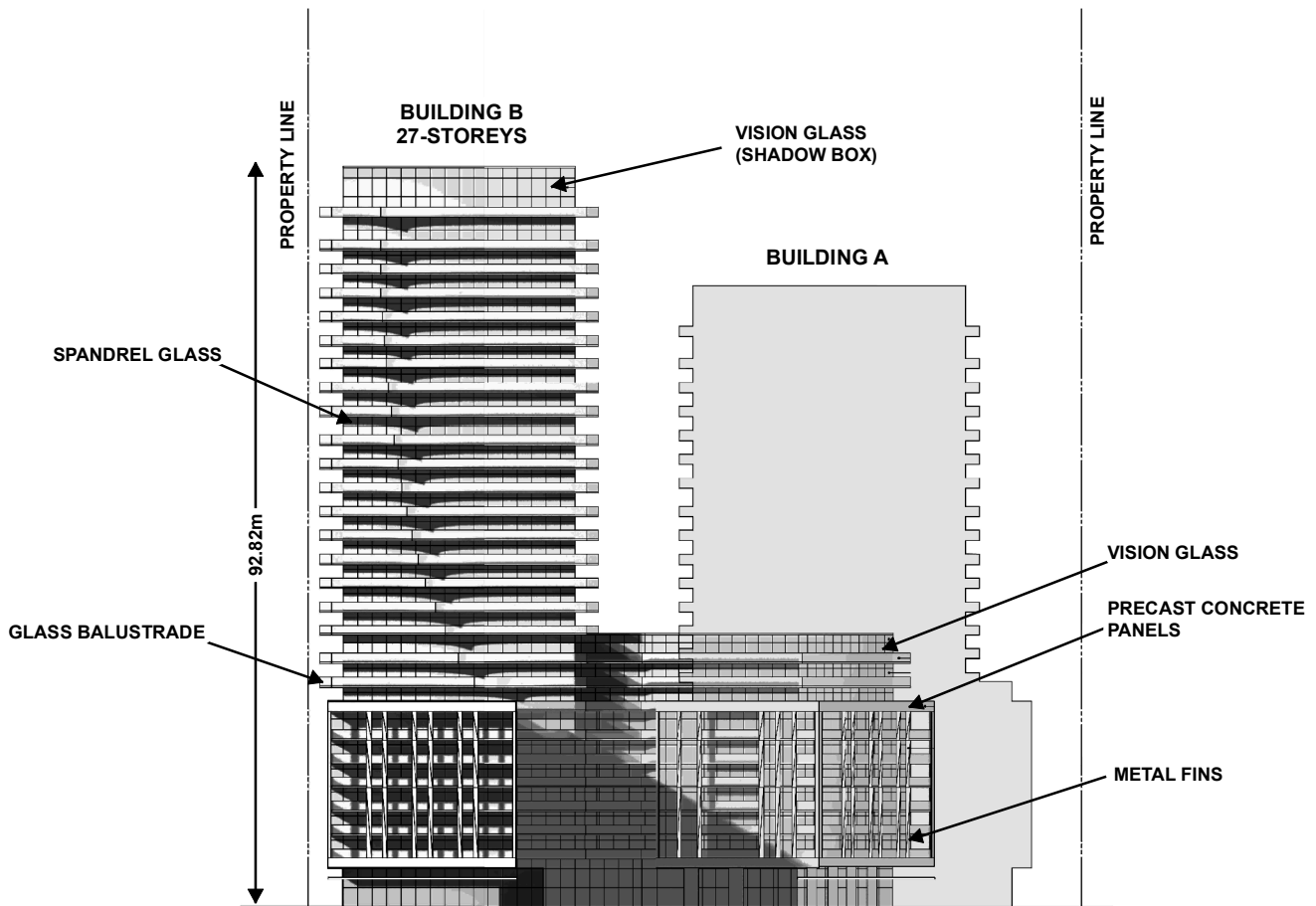
BUILDING B - EAST ELEVATIONS
