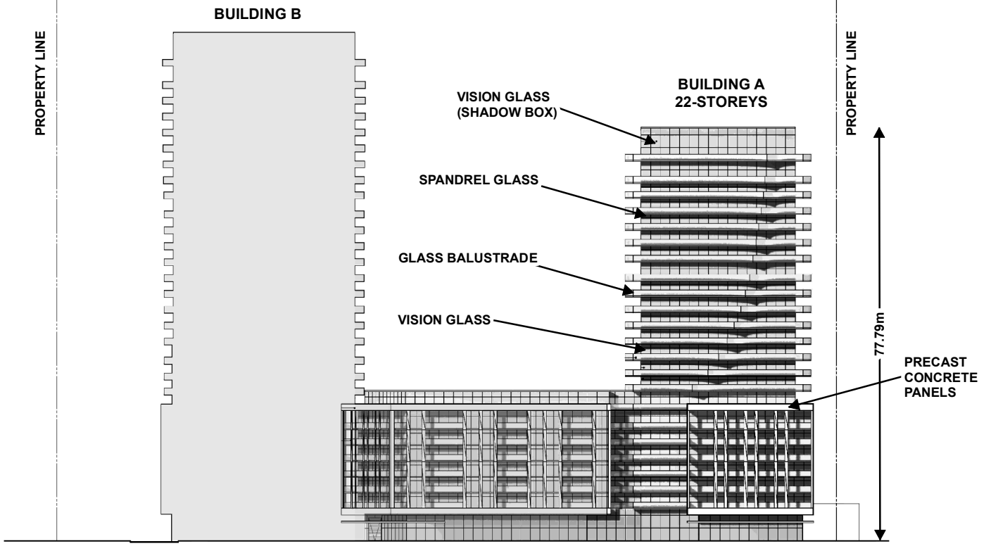
BUILDING A - SOUTH ELEVATIONS
