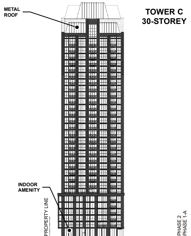
WEST ELEVATION
