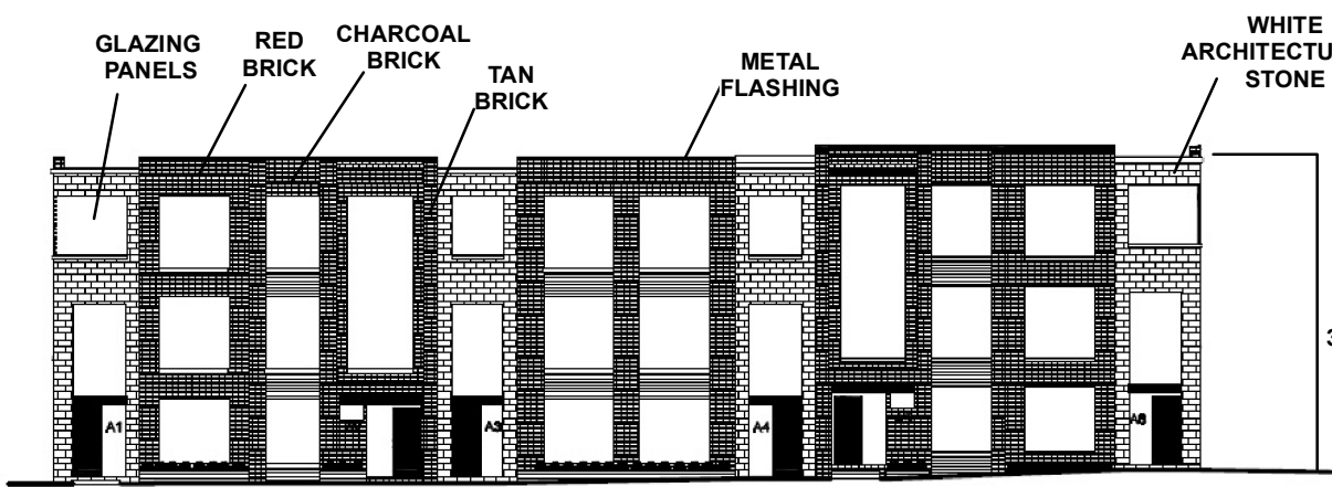
EAST ELEVATION
