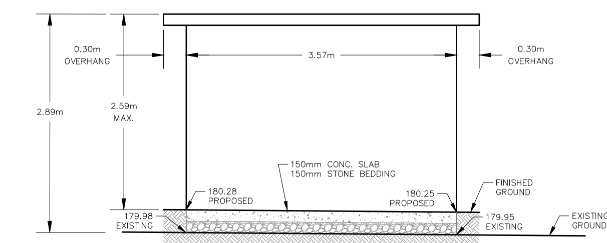
SHED FRONT ELEVATION SCALE: 1:50
