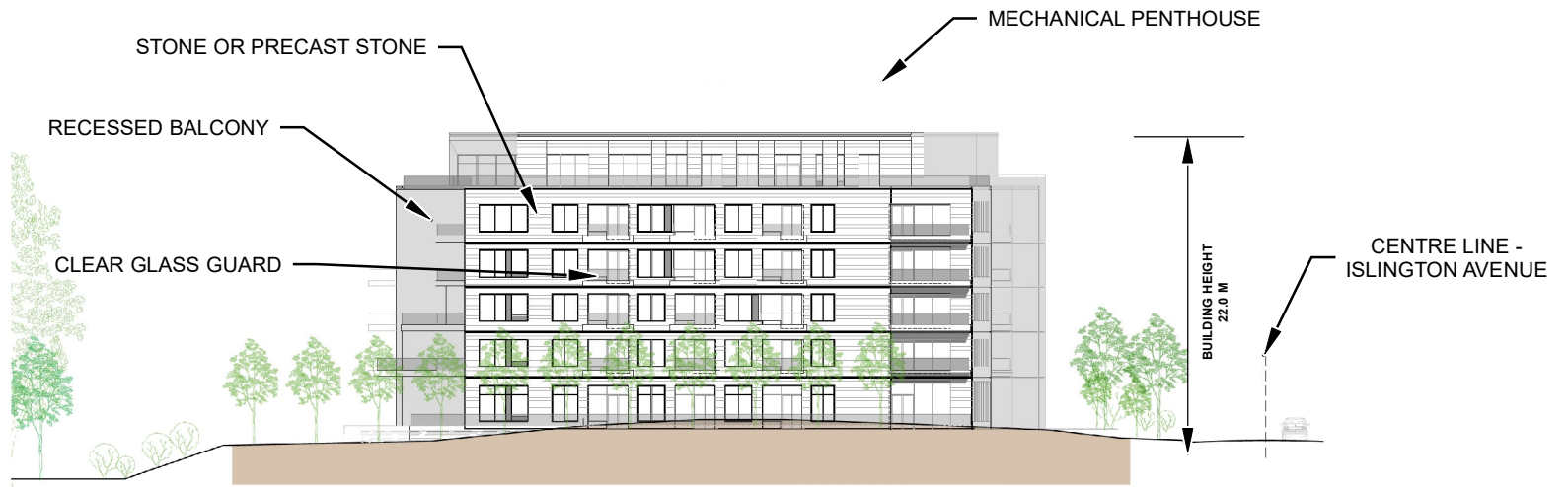
NORTH ELEVATION
