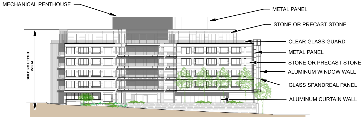
WEST ELEVATION (FACING ISLINGTON AVENUE)
