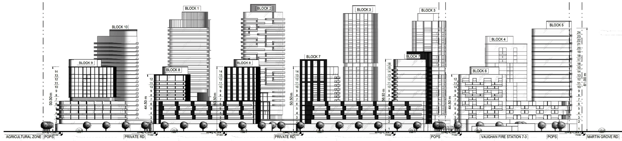
SOUTH ELEVATION
