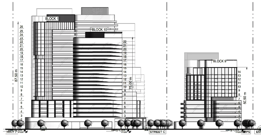
WEST ELEVATION
