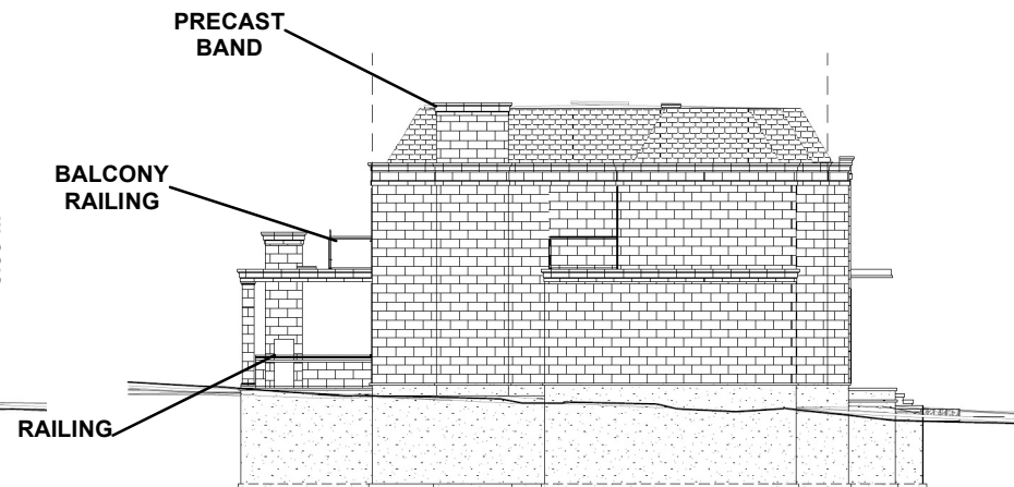
DWELLING A - WEST ELEVATION
