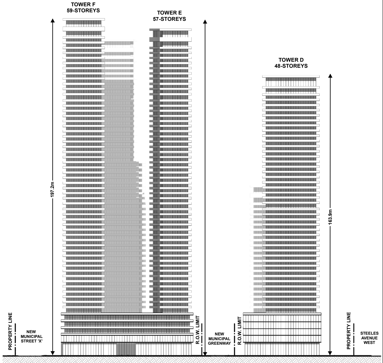
WEST ELEVATIONS - FACING STREET 'D'
