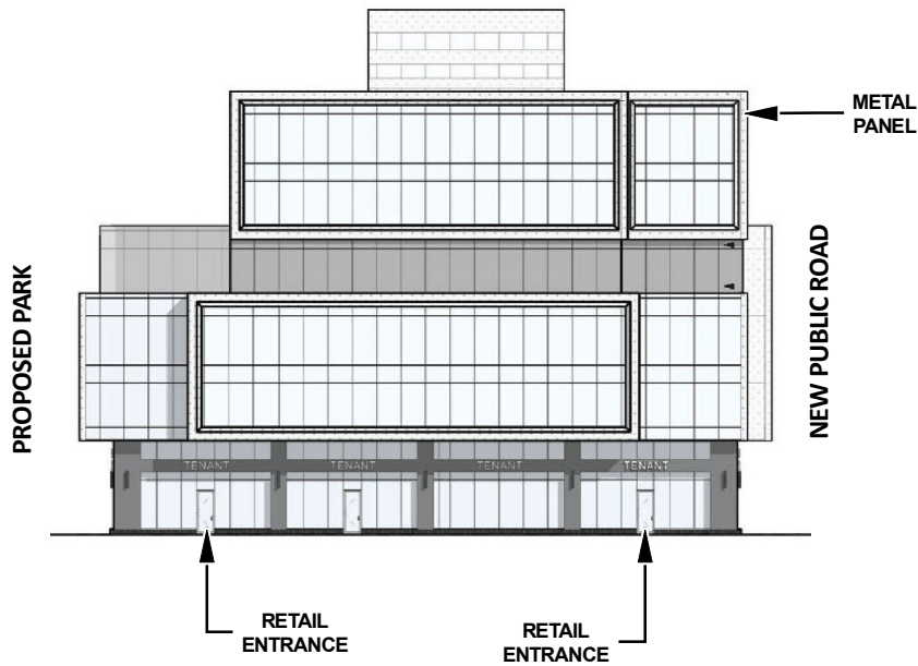
WEST ELEVATION
