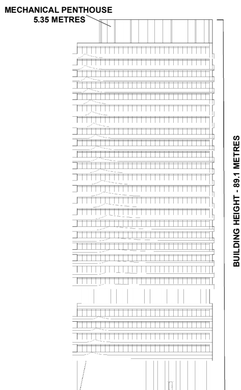
NORTH ELEVATION
