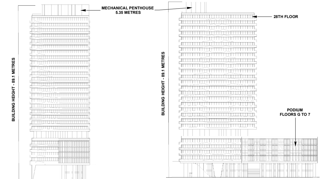
NORTH ELEVATION
