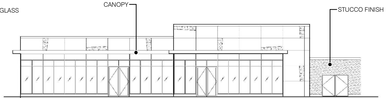
WEST ELEVATION
