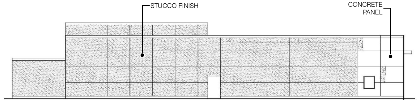
EAST ELEVATION
