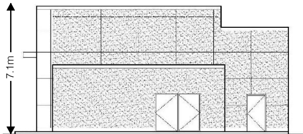
SOUTH ELEVATION
