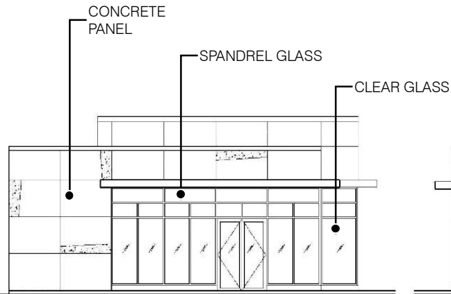
NORTH ELEVATION (FACING REGIONAL ROAD 7)
